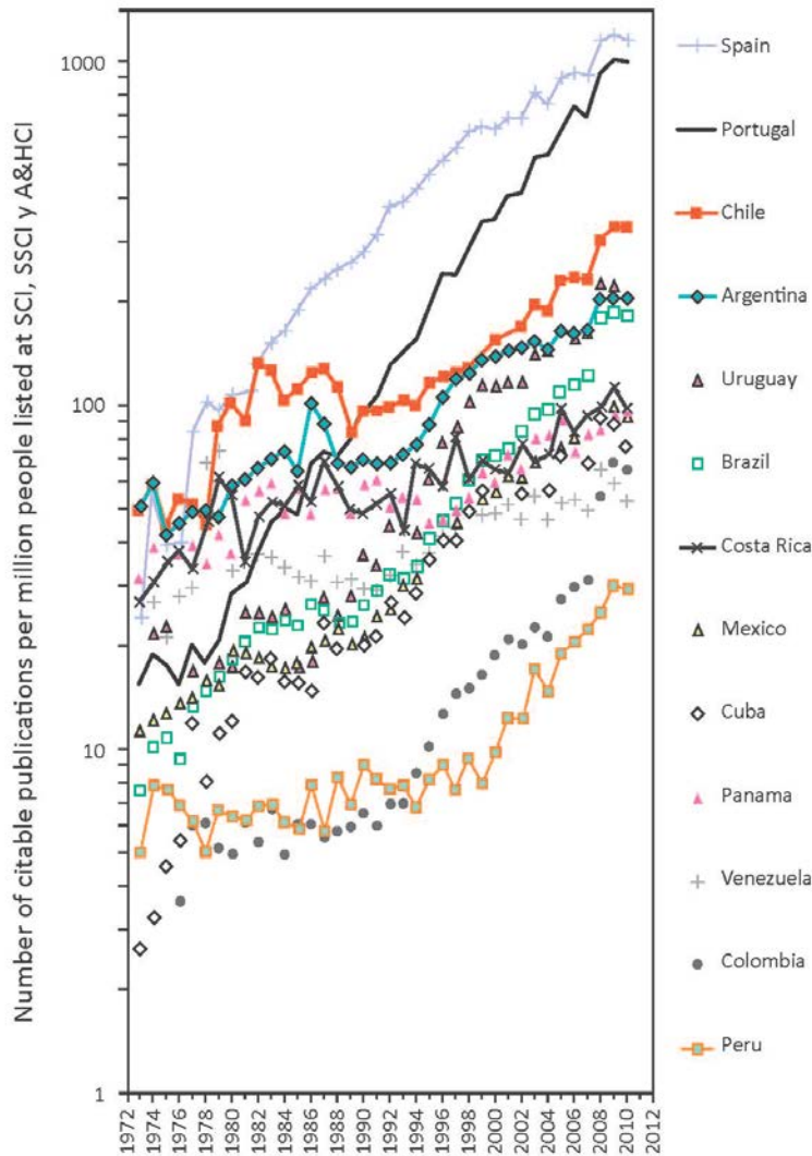
Fig. 2. Number of citable publications per million people for the Iberoamerican countries with the largest number of publications.
